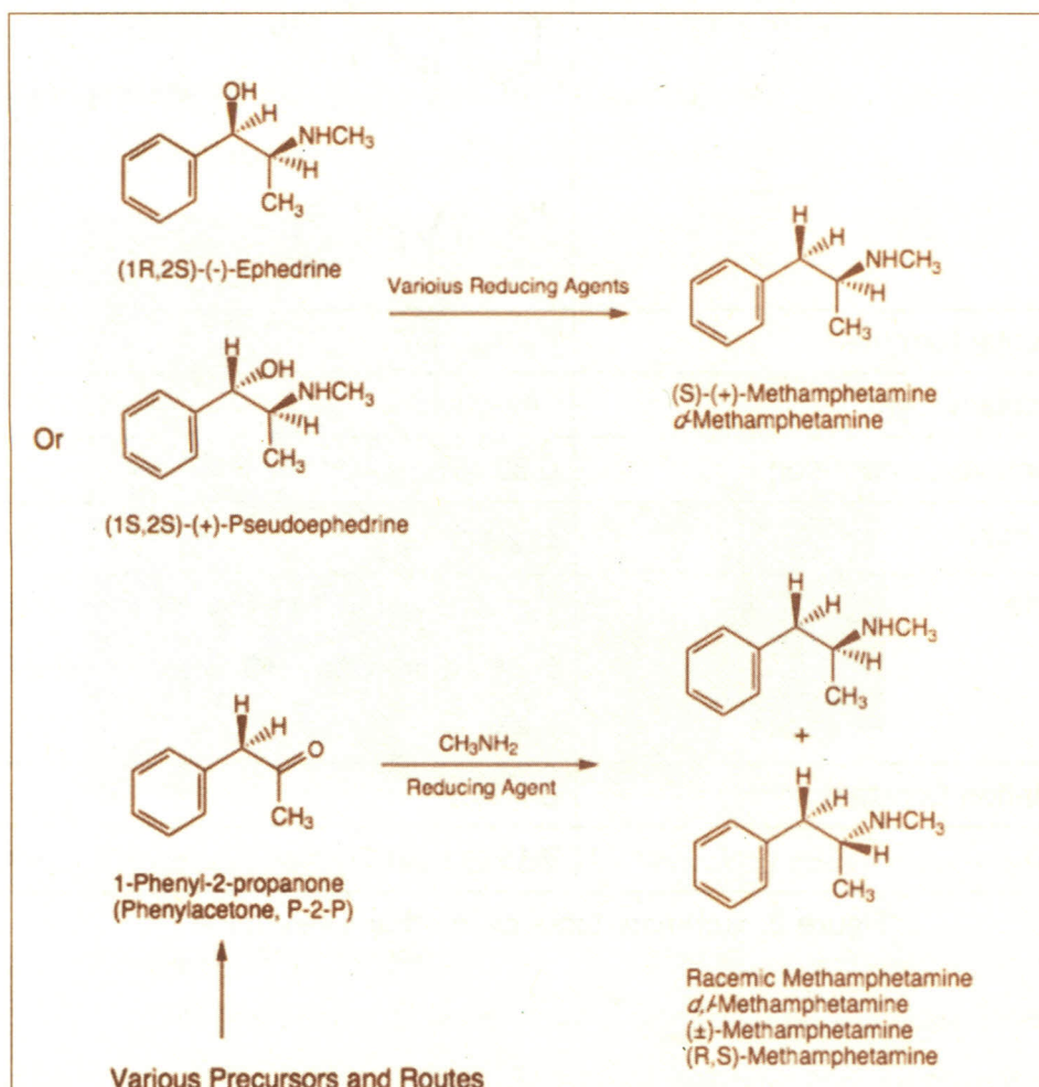
Figure 1. synthesis of Methamphetamine [ source : Human Pharmacology of the methamphetamine stereoisomers write by John Mendelson, Naoto Uemura .( 2011 ) ]
